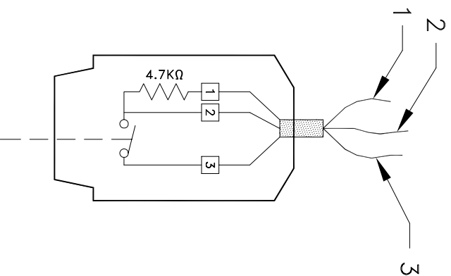
ELECTRICAL DIAGRAM
