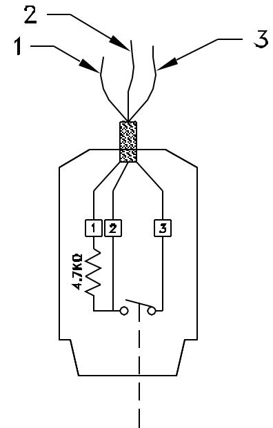
ELECTRICAL DIAGRAM
